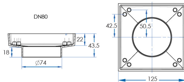
Cover Plate
